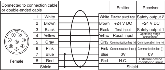
Single-end Connector Cable Internal wiring diagram (F39-JD□A)
