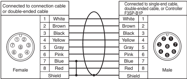
Double-end Connector Cable Internal wiring diagram (F39-JD□B)
