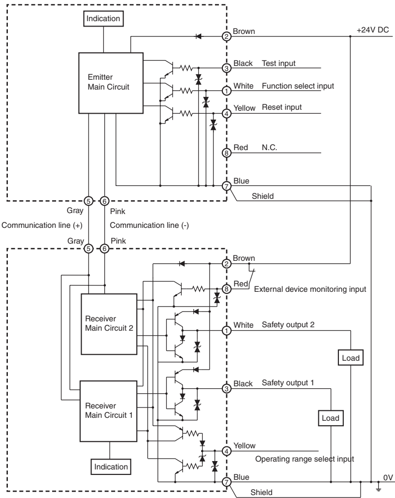
Single-end Connector Cable Internal wiring diagram (F39-JD□A)
