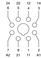
Terminal Arrangement
